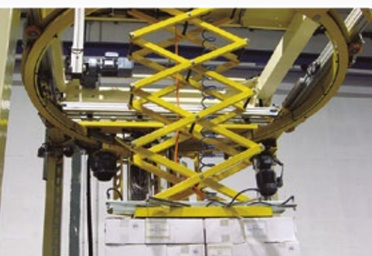
Motorized hold down plate
