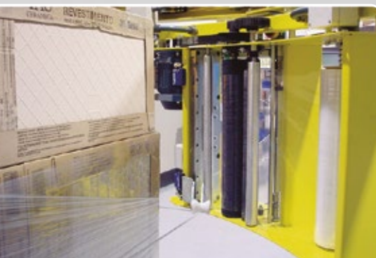
Roping device
